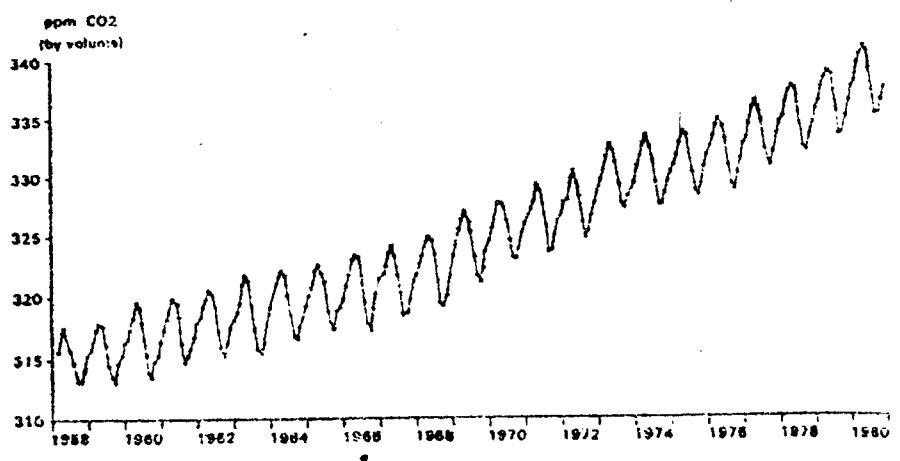
Figure Monthly average carbon dioxide concentrations at Mauna Loa Observatory
