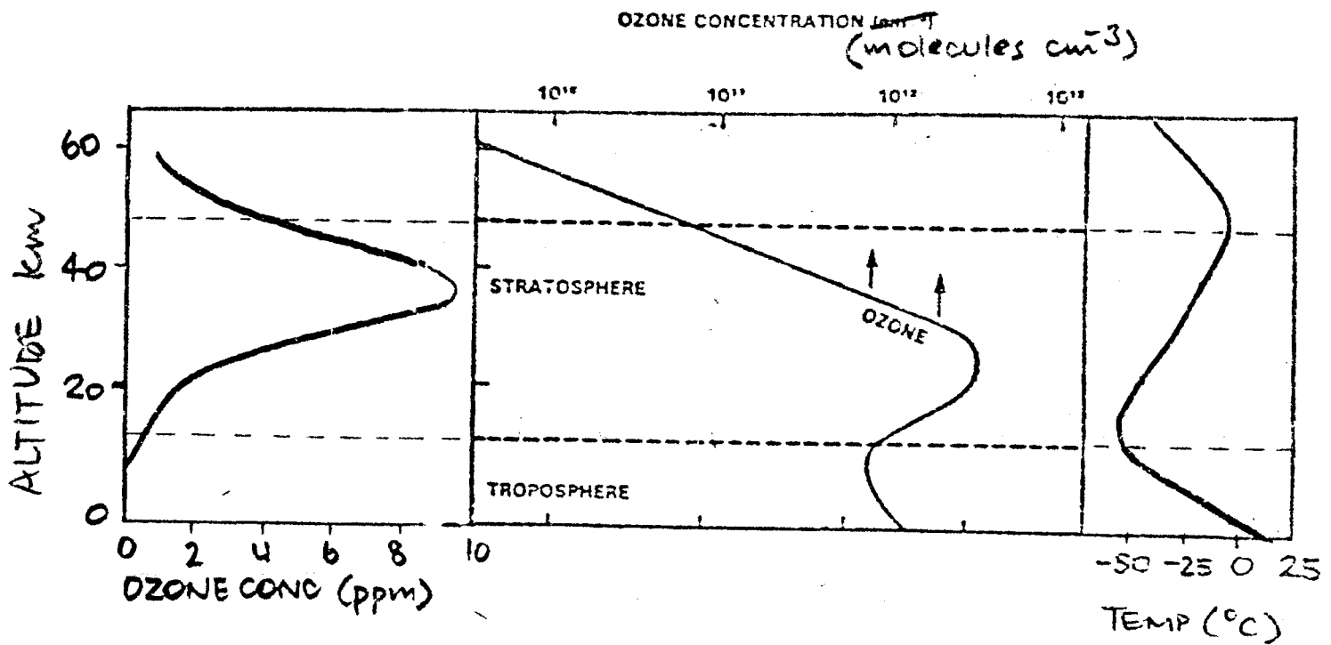
FIGURE 1 Temperature profile and ozone distribution in the atmosphere
