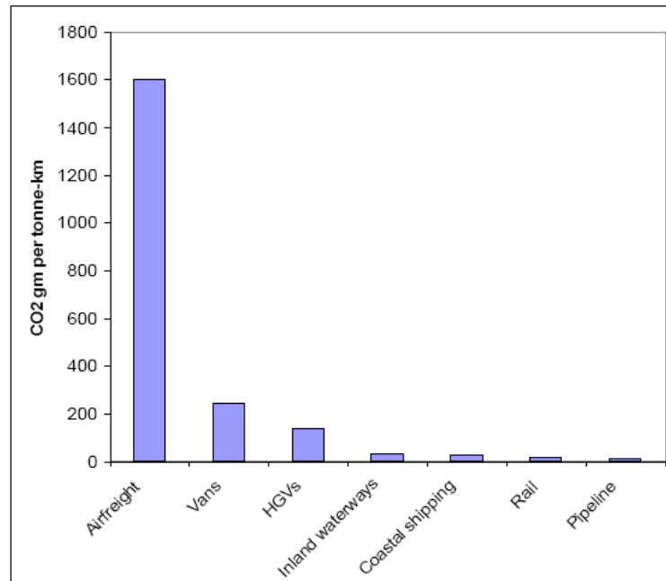
Fig. 7-1: Typical CO2 Emissions for Various Transport Options (McKinnon)
