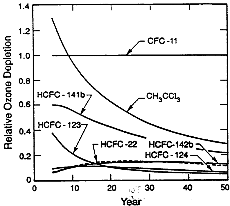
Figure 4.1. Calculated column ozone change following a pulsed input of 5 \times 10^9 kg (for one year) of specified gas (DuPont 1-D model).
