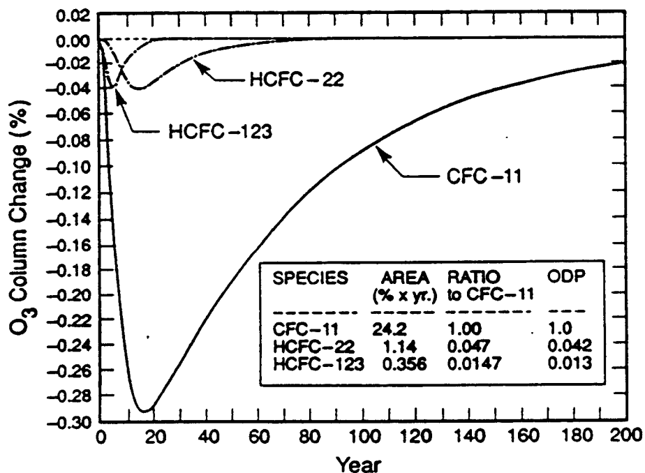
Figure 4.2. Calculated time-dependent change in relative ozone column depletion following a step change in emission of halocarbons (DuPont 1-D model).
