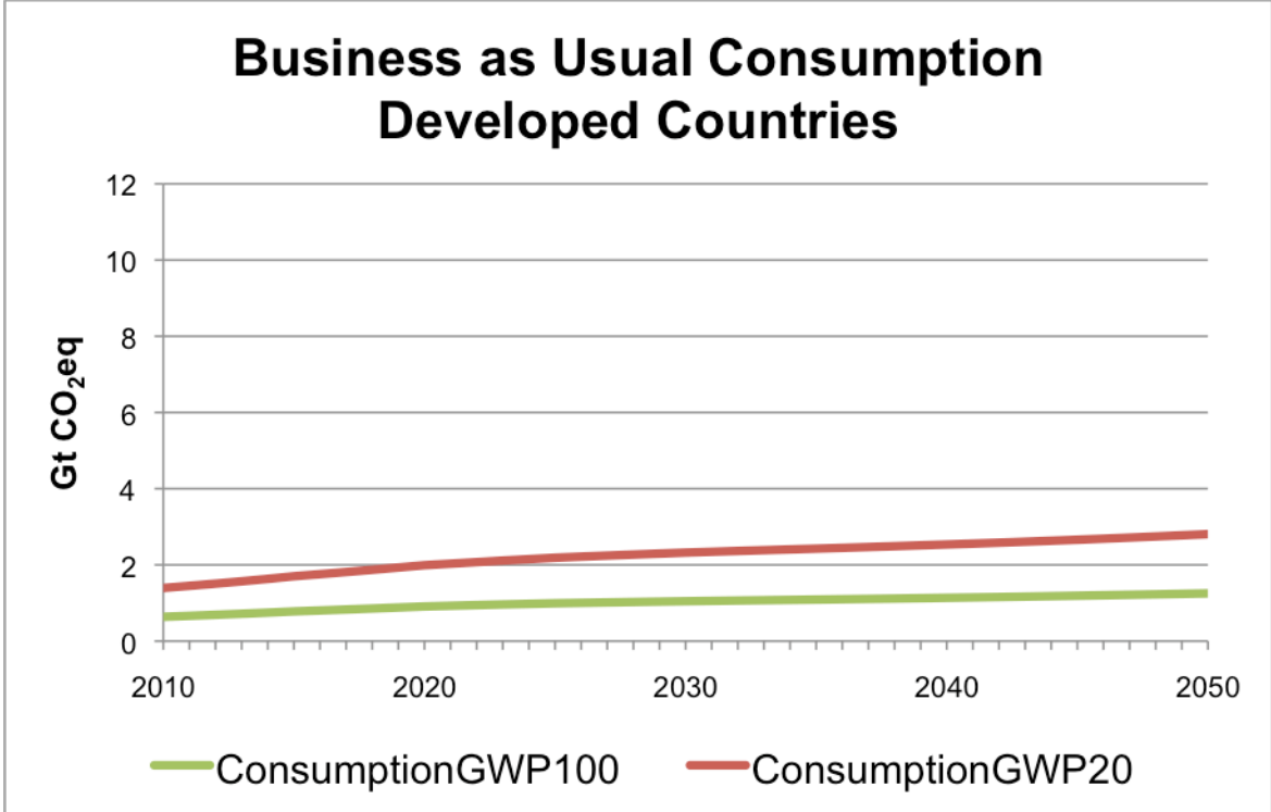
Graph 2: HFC consumption in developed (A2) countries (2010-2050, BAU scenario)
