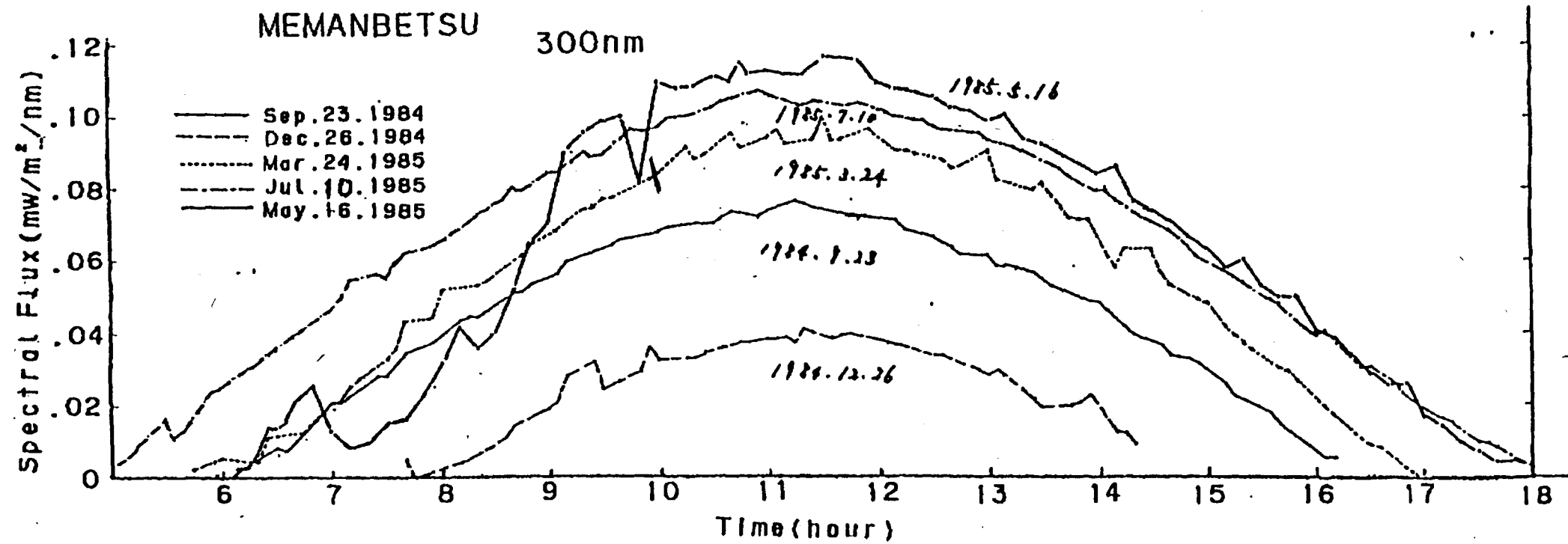
Fig. 4(d) Diurnal variation of solar radiation at 300 nm, Memanbetsu ( 43.9^{\circ}\text{N} )
