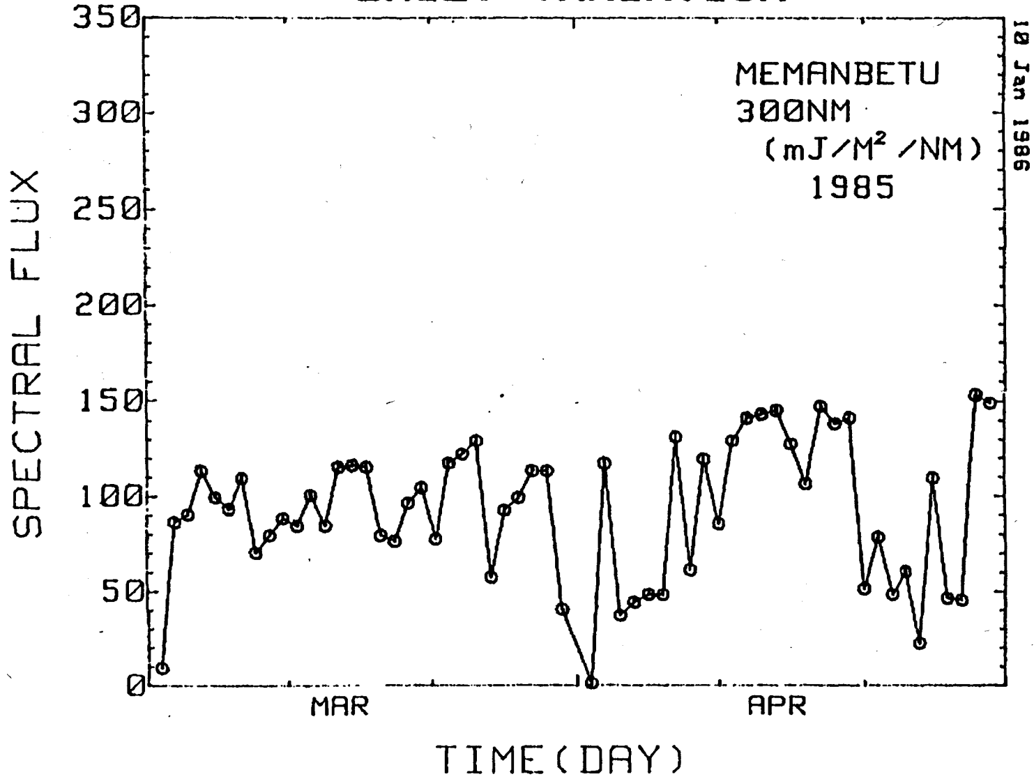
Fig. 4 (a) Daily variation of solar radiation at 300 nm at Memanbetu (43.9°N)
