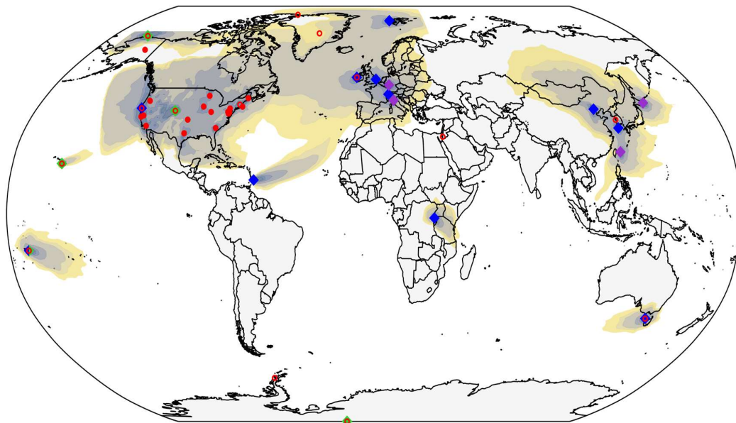
Figure 1. Map of Advanced Global Atmospheric Gases Experiment (AGAGE) high-frequency measurement stations (blue diamonds), AGAGE affiliated high-frequency measurement stations (purple diamonds), National Oceanic and Atmospheric Administration (NOAA) high-frequency measurement stations (green diamonds), NOAA daily flask-sampling locations (red filled circles) and NOAA weekly flask-sampling locations (red open circles) for monitoring atmospheric substances controlled by the Montreal Protocol. Modelled 2,4 annual “footprint” sensitivities are shown for the plotted high-frequency in-situ measurement and daily flask sampling locations (except for the South Pole, central Alaska, and parts of the Beaufort Sea north of Alaska). Sensitivity contours begin at the approximate limit where quantitative estimates of emissions can be made and increase exponentially toward the station locations.
